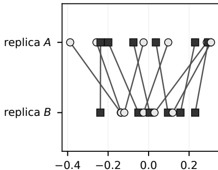
within-sign matching multiplier -1
