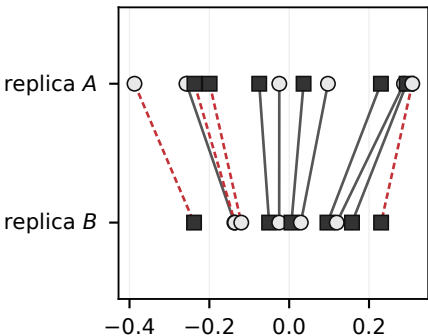
rank matching multiplier -\text{sgn}(m_{A,i})\text{sgn}(m_{B,i})
