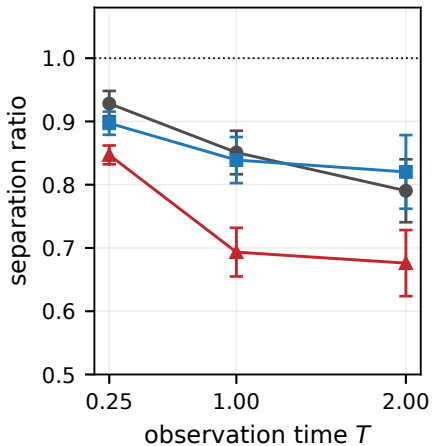
matched-pair separation ratio
