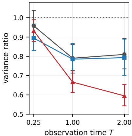
integrated variance ratio
