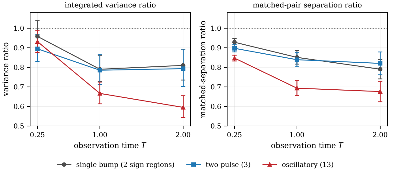
Fig. 3 The left panel shows the integrated variance ratio of sign-switched to within-sign pairing across three fixed profiles and three observation times (Table 3). The right panel shows the matched-pair separation ratio at a fixed paired state (Table 4), which cannot exceed 1 by Remark 3.9. It measures the increase in distance from constraining the matching to respect sign classes, not the variance mechanism.
