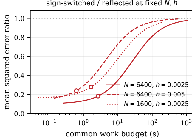
Fig. 5 Model mean squared error ratio (4.5) at equal work, at three archived (N, h) cells of the two-pulse problem with 64 paired seeds. The shared squared bias b^2 is the same estimate in numerator and denominator, as Corollary 3.3 requires. Circles mark W = C_{\text{switch}} V_{\text{switch}} / b^2 . Three configurations do not establish a convergence rate or independently resolve the effects of N and h .
