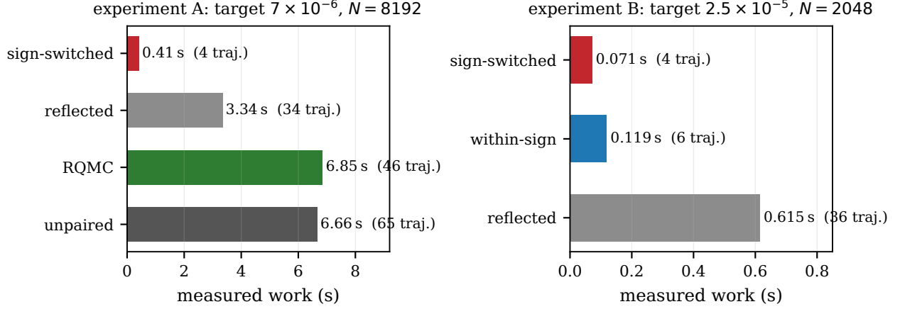
Fig. 4 Measured work to attain a common expected-error target in the two held-out experiments, which have different targets, different N and different arms and are not to be pooled. The left panel reports experiment A (Table 5), and the right reports experiment B (Table 6).
