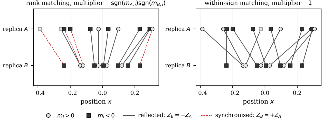
Fig. 1 The two matchings applied to the same paired state immediately before the tenth diffusion stage of the interleaved-sign configuration, with N = 12 . The left panel pairs particles of equal spatial rank and synchronizes the increments of unlike-sign pairs. The right panel restricts partners to the same sign and reflects every pair. The state is identical in both panels, so the difference in separation comes only from the matching rule. Both rules preserve each replica’s law (Proposition 3.1).
