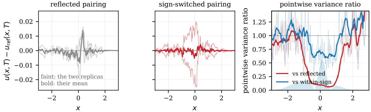
Fig. 2 Two-pulse Burgers, N = 8192 , 48 replicates, from the independently replayed archive. The left and centre panels show the pointwise error of each replica (faint) and of their mean (bold) on one replicate. The right panel shows the ratio of pointwise variance of the sign-switched pair mean to that of the reflected (red) and within-sign (blue) pair means. Thin lines are the raw ratios over 48 replicates and thick lines a 13-point running mean. The shaded profile is |\partial_x u_{\text{ref}}| , scaled to the panel.
