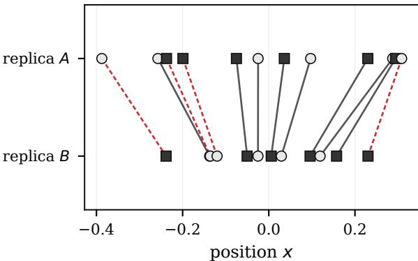
rank matching, multiplier -\text{sgn}(m_{A,i})\text{sgn}(m_{B,i})
