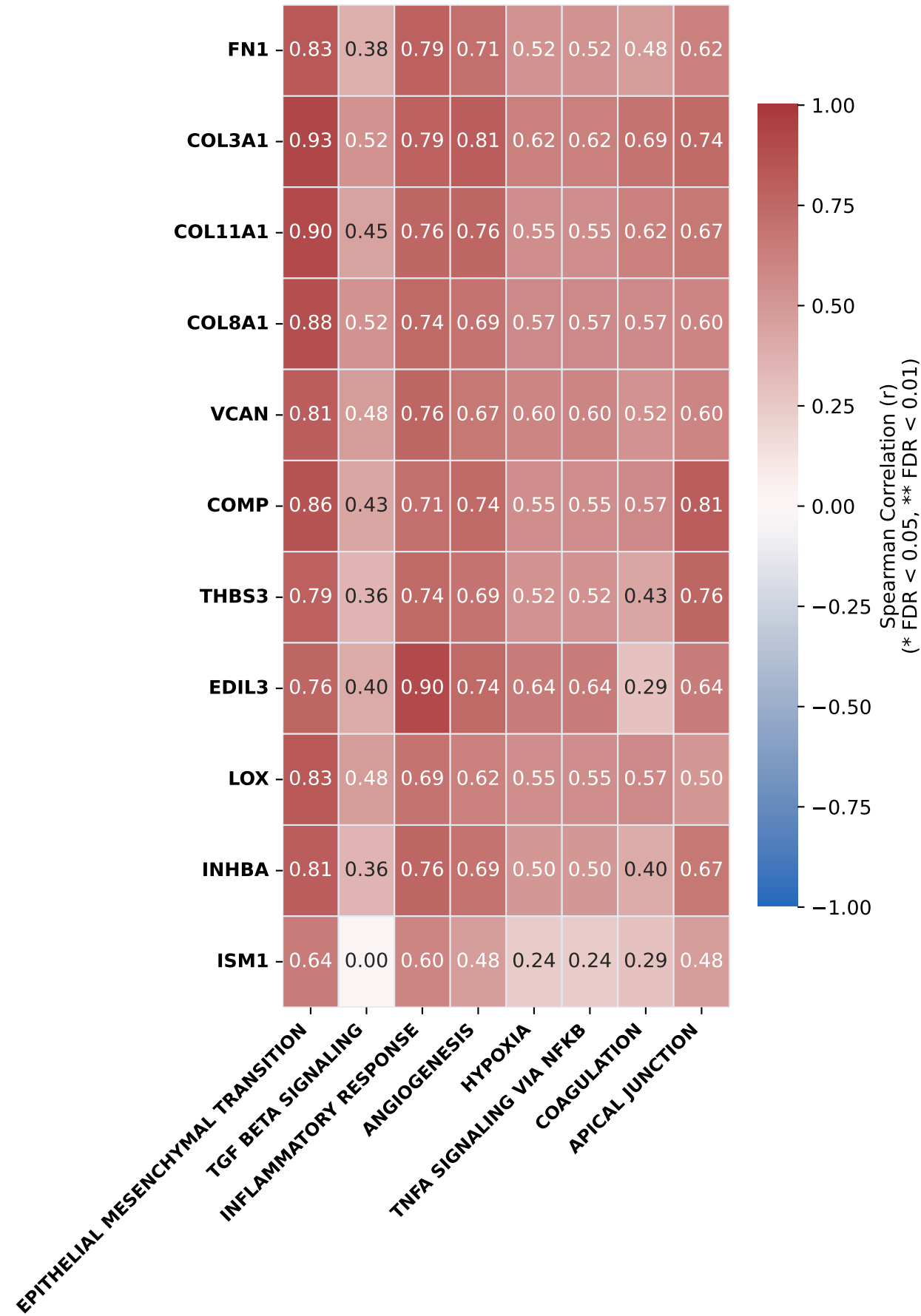
C. Circularity-Corrected ssGSEA Correlation (Hub Gene Removed from Gene Set; N = 8)
