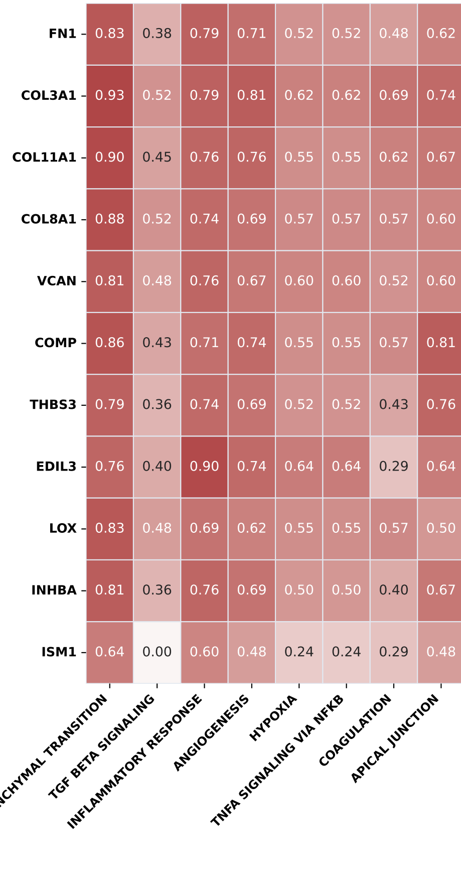
B. Standard ssGSEA Score Correlation (Unadjusted; Potential Circularity)
