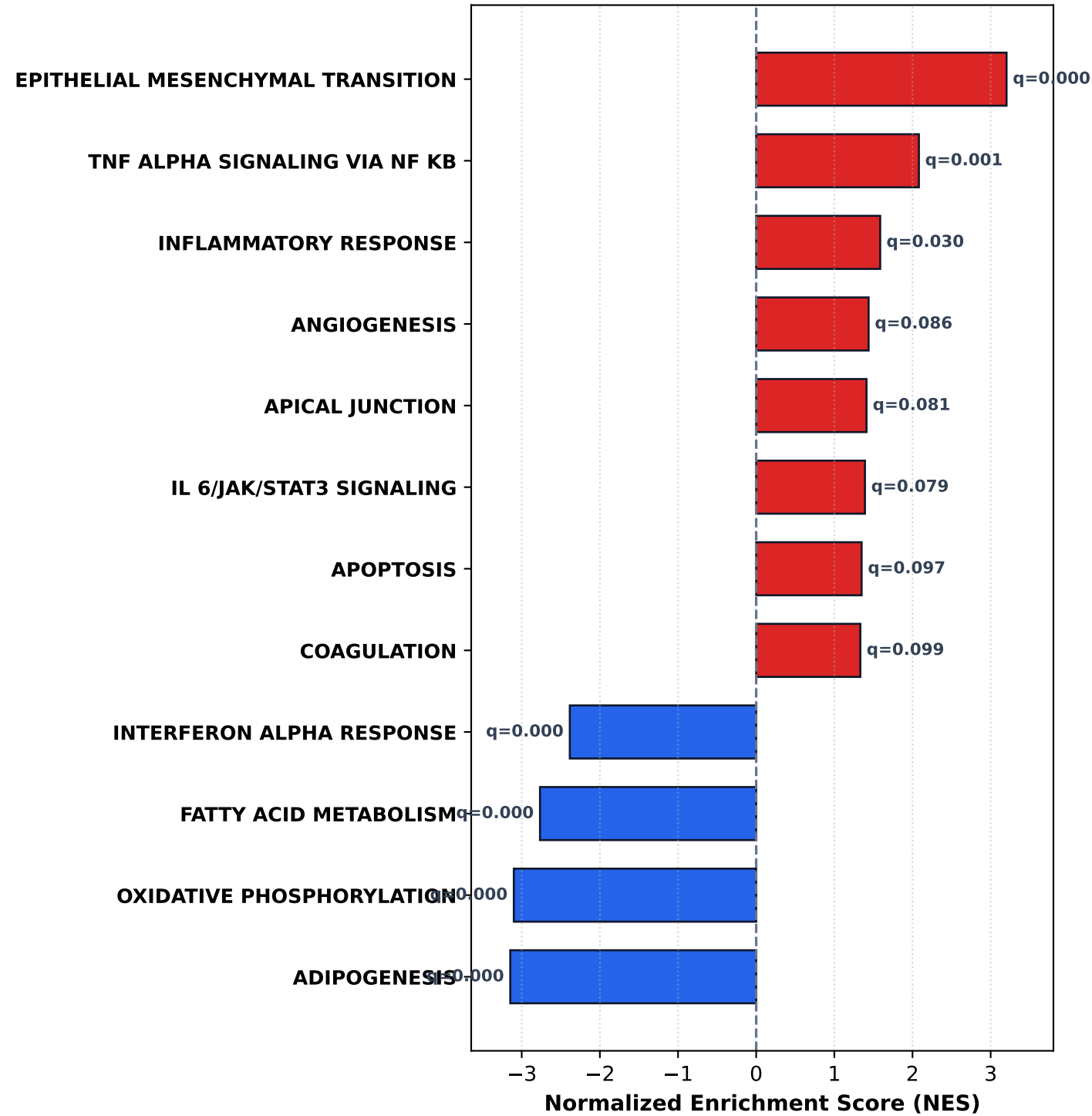
A. True Preranked GSEA (MSigDB Hallmark v2020) Ranked by Moderated t-Statistic (EPS vs Control)
