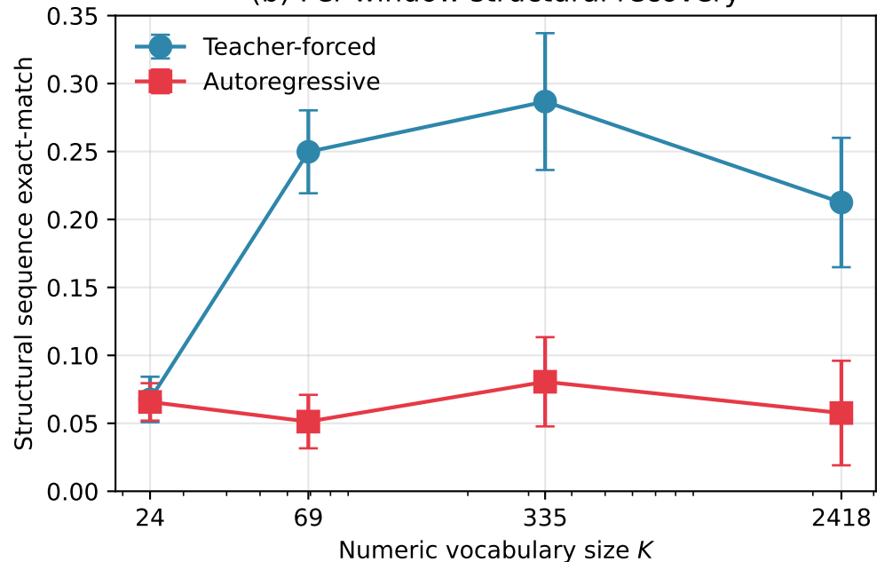
(b) Per-window structural recovery
