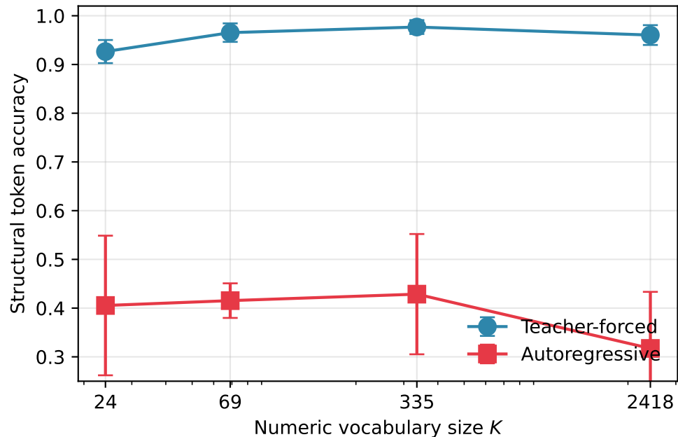
(a) Per-token structural recovery
