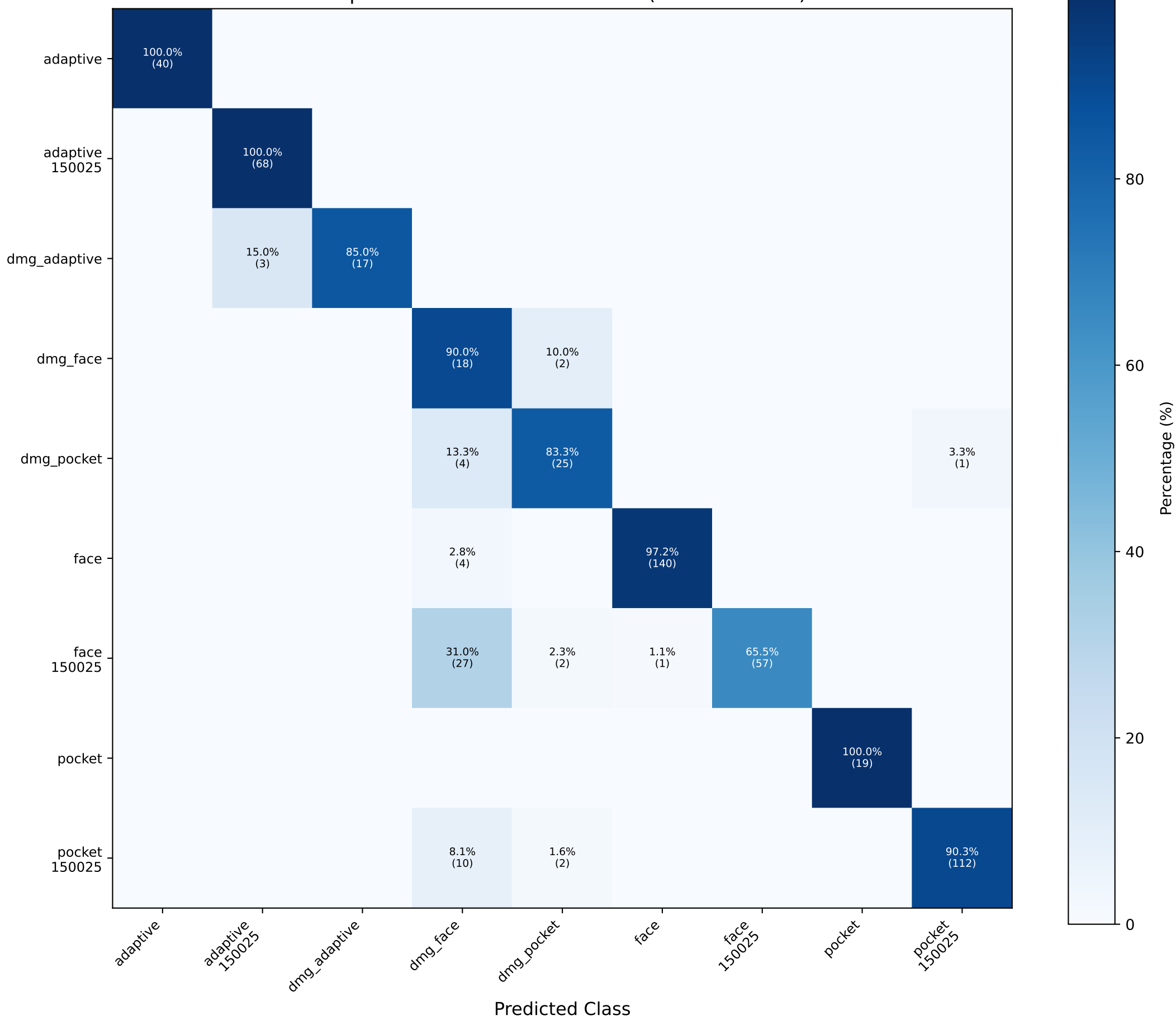
Sequence-Level Confusion Matrix (% of true class)
