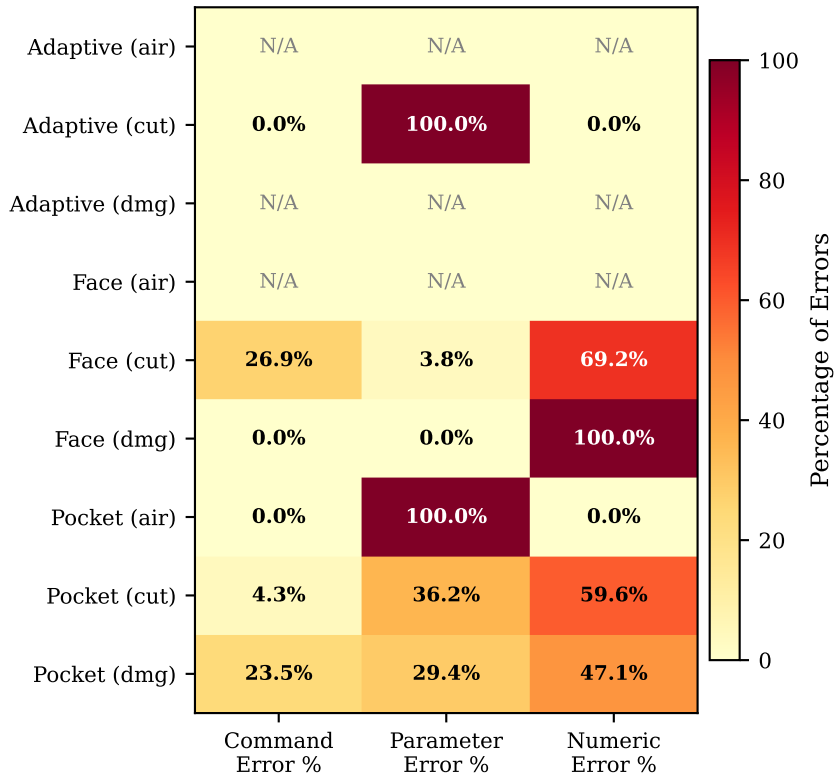
Error Distribution by Token Type per Class
