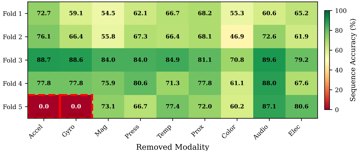
Sequence Accuracy by Removed Modality and Fold
