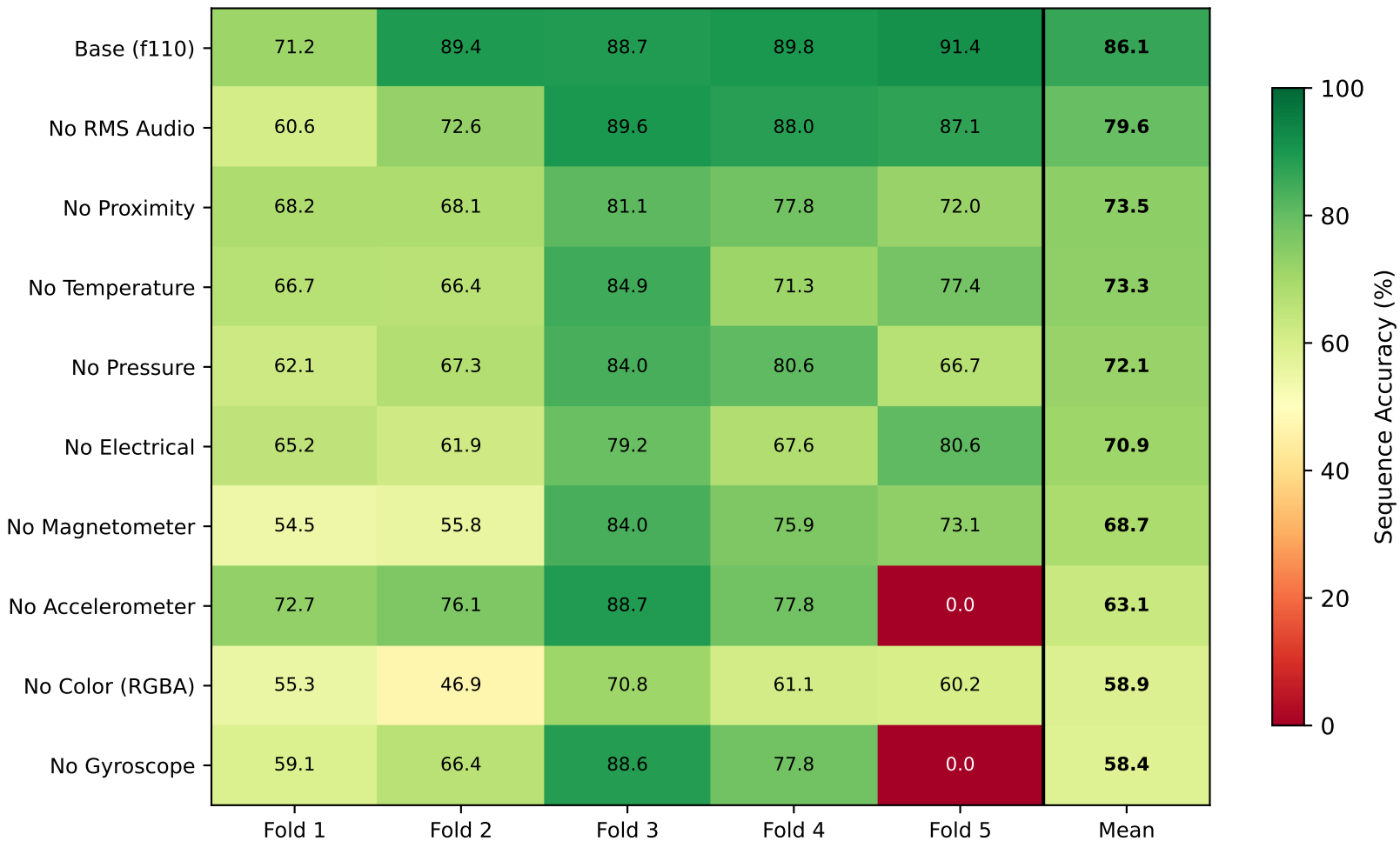
Modality Ablation: Per-Fold Sequence Accuracy (%)
