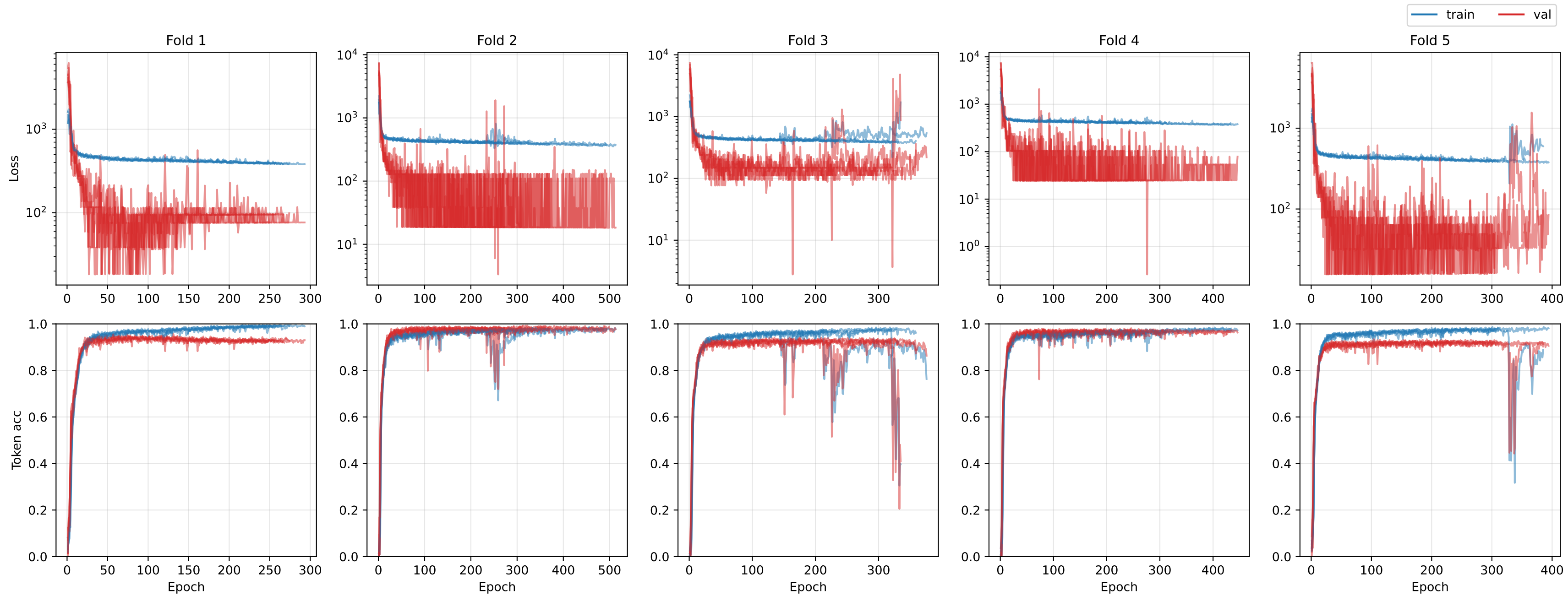
V7 Multi-Seed Training Curves (5 seeds \times 5 folds)
