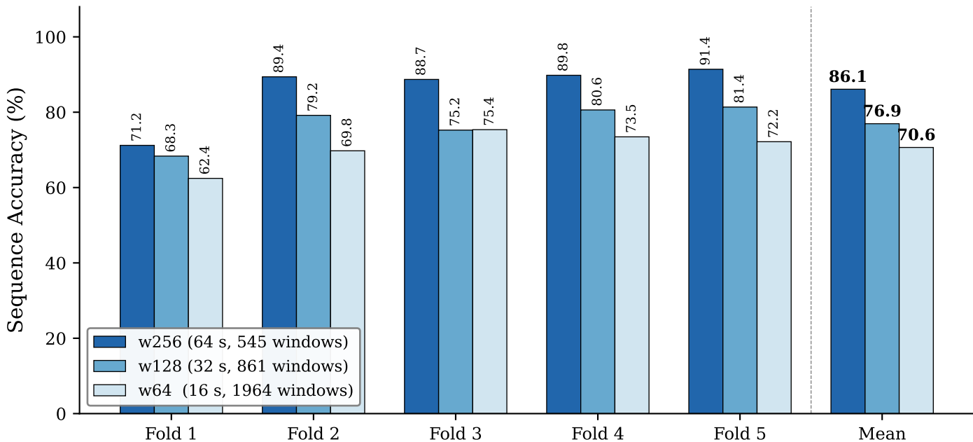
Window Size Ablation: Per-Fold Sequence Accuracy
