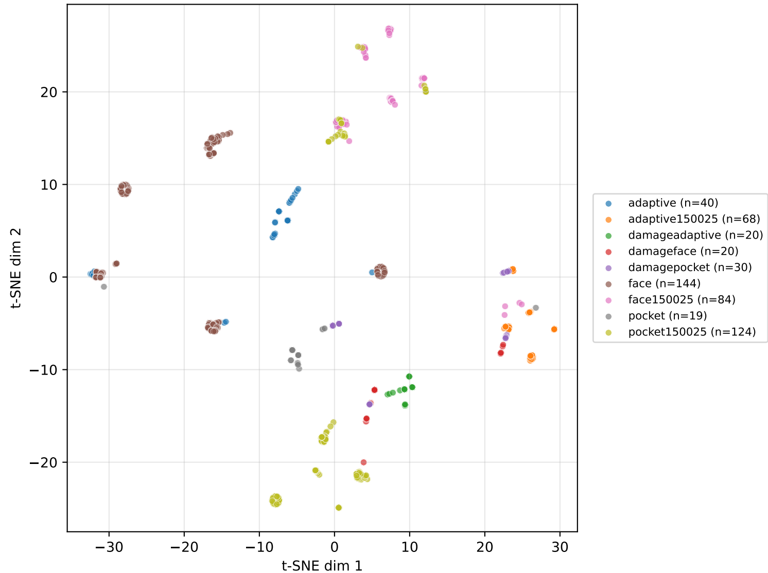
t-SNE of frozen encoder memory (mean-pooled over time), coloured by operation class — 549 test samples, 5 folds
