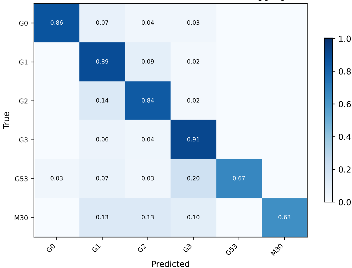
Command head — confusion matrix (5-fold aggregate)
