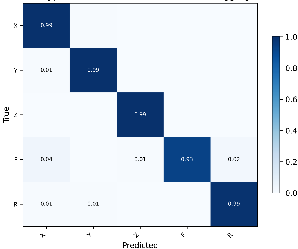
Param-type head — confusion matrix (5-fold aggregate)
