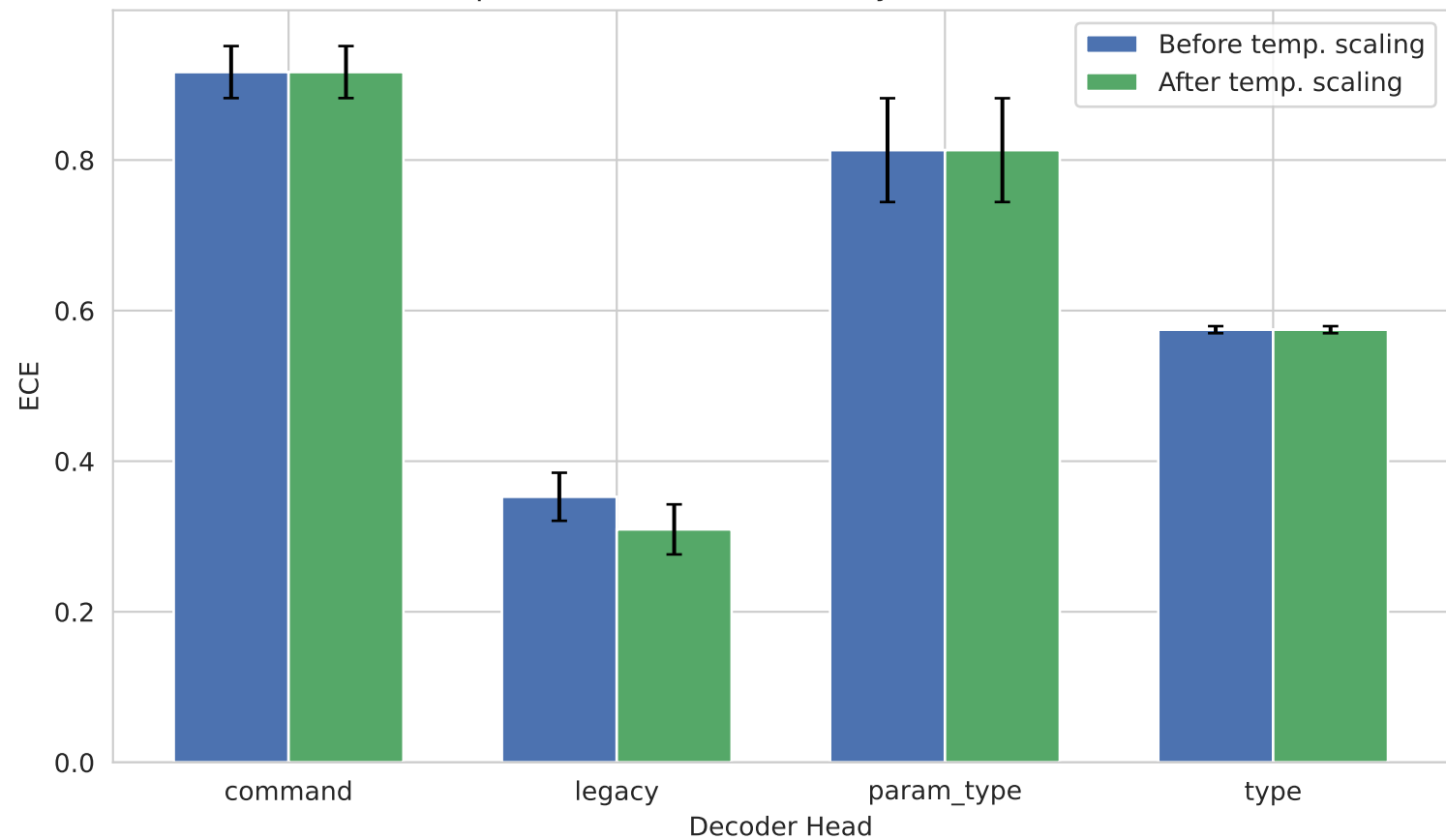
Expected Calibration Error by Decoder Head
