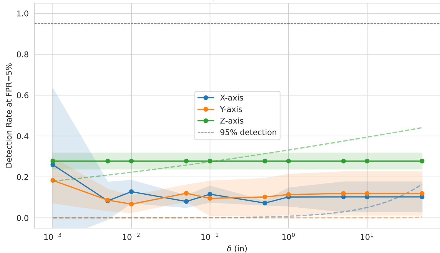
Graded Coordinate Injection: Detection Rate vs Delta
