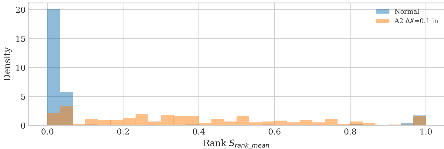
(b) Rank Score Distribution: Normal vs. A2 Coord \Delta X=0.1 in
