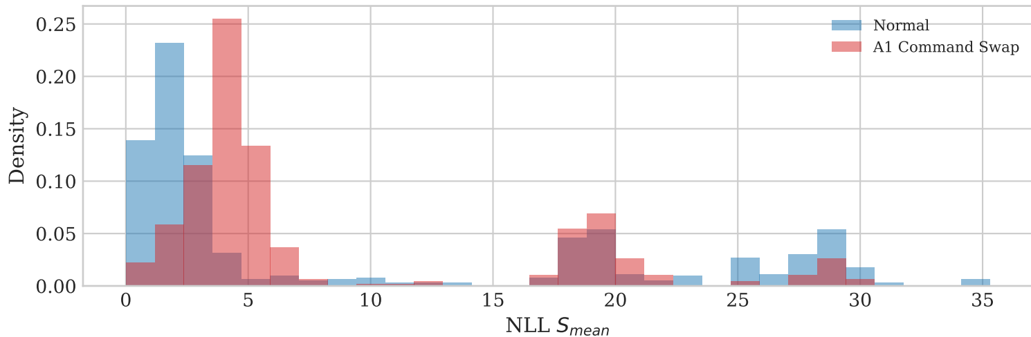
(a) NLL Score Distribution: Normal vs. A1 Command Swap
