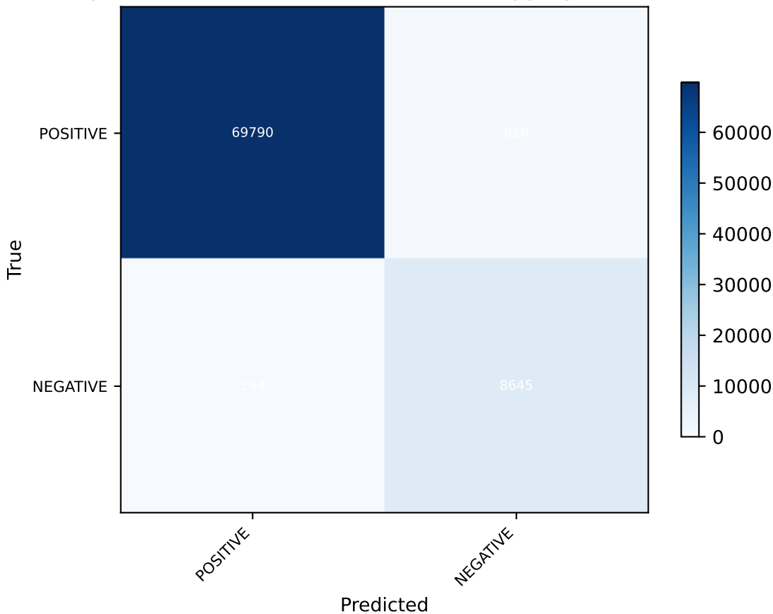
Sign head — confusion matrix (5-fold aggregate counts)
