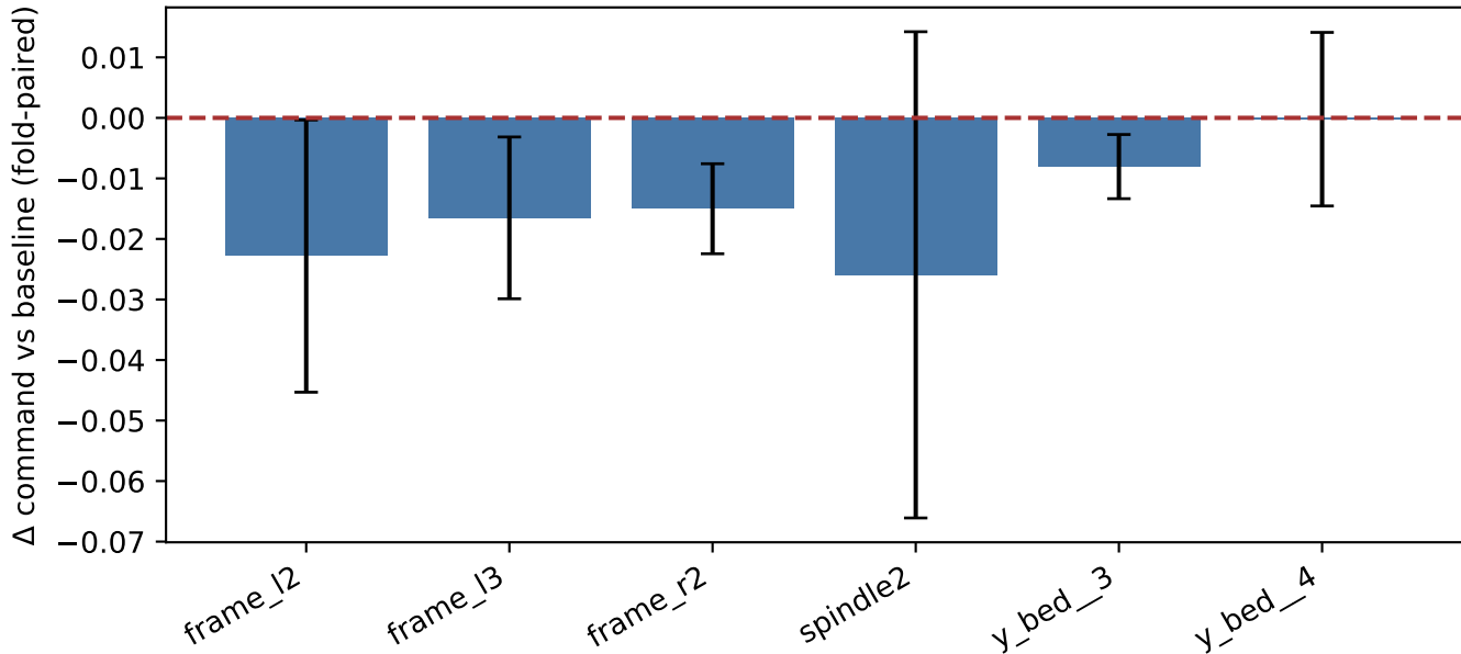
Leave-one-sensor-out encoder retraining (full-window, 5-fold)
