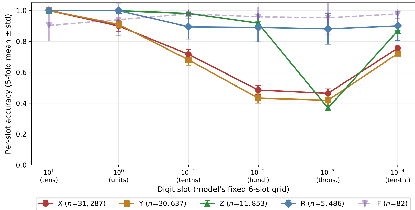
Per-axis per-slot accuracy: Z's recovery profile is structurally different from X/Y; R's profile is uniformly high
