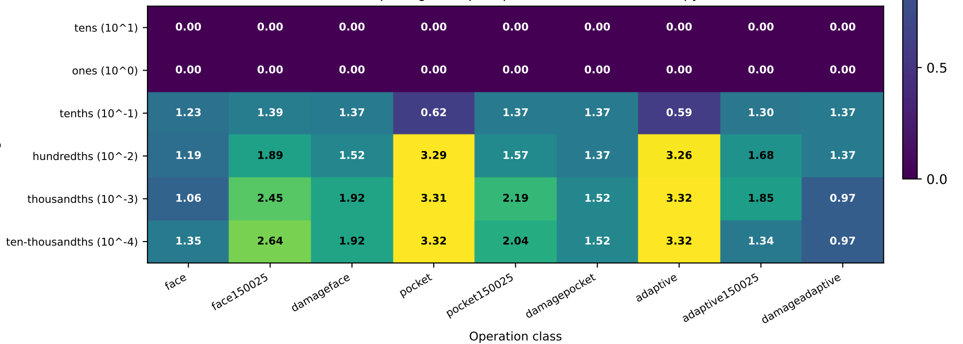
Z axis: per-digit-slot per-operation-class source entropy
