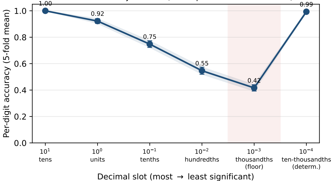
Numeric-recovery bathtub (float-epsilon-corrected retrain)
