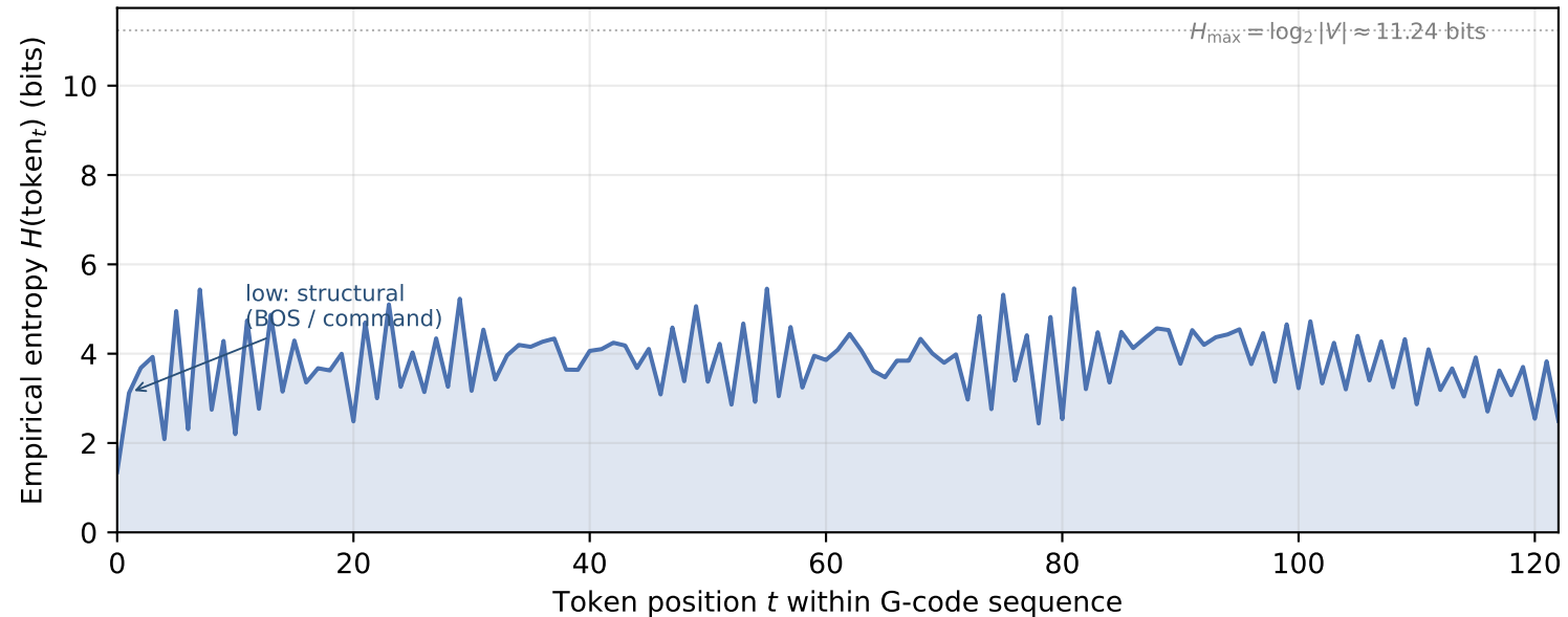
Per-position source entropy of the V8 token stream
