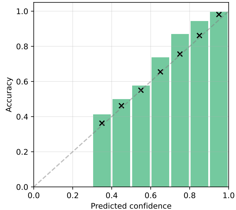
param_type head ECE=0.020, MCE=0.114
