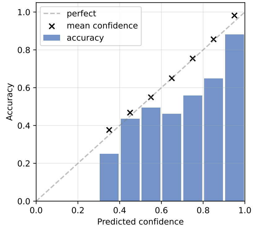
command head ECE=0.122, MCE=0.207
