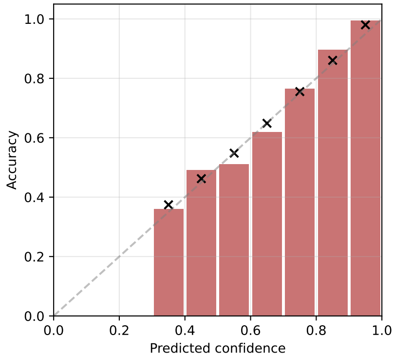
type head ECE=0.015, MCE=0.037
