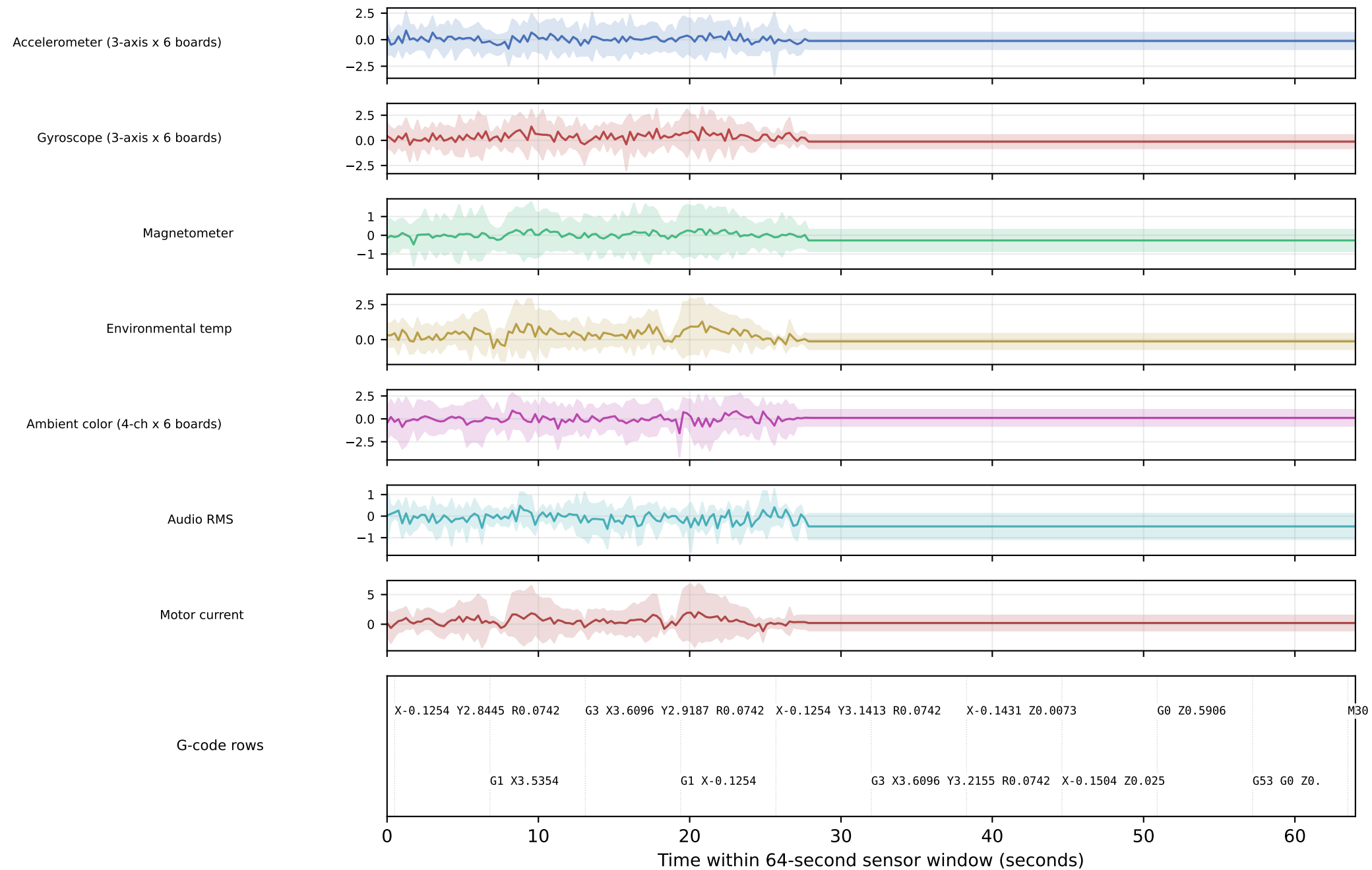
Multi-modal sensor window (64 s, 4 Hz, 256 samples × 98 channels) and aligned G-code rows. Operation class: face150025, source: face150025_001_aligned, 11 G-code rows
