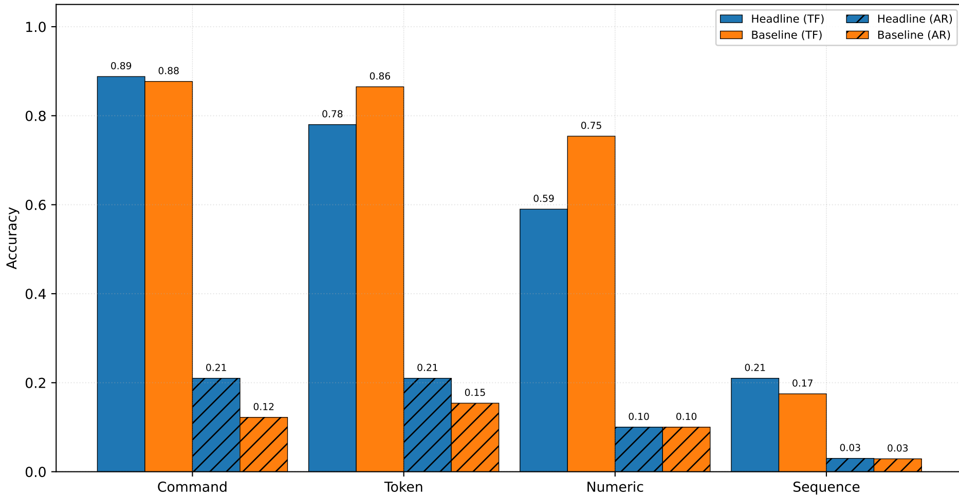
Seq2Seq baseline vs headline: TF parity, AR divergence
