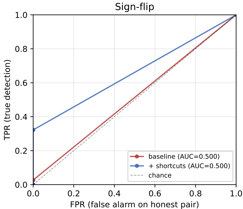
Tamper-detection ROC curves (autoregressive predictions, 5-fold pooled)
