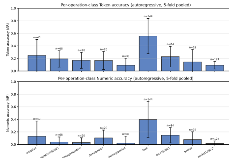
Figure 2. Per-operation-class AR token (top) and numeric (bottom) accuracy, 5-fold pooled; error bars are within-class std across test samples. The open-vocabulary LOCO counterpart chart is released as figures/loco_per_holdout.pdf.
