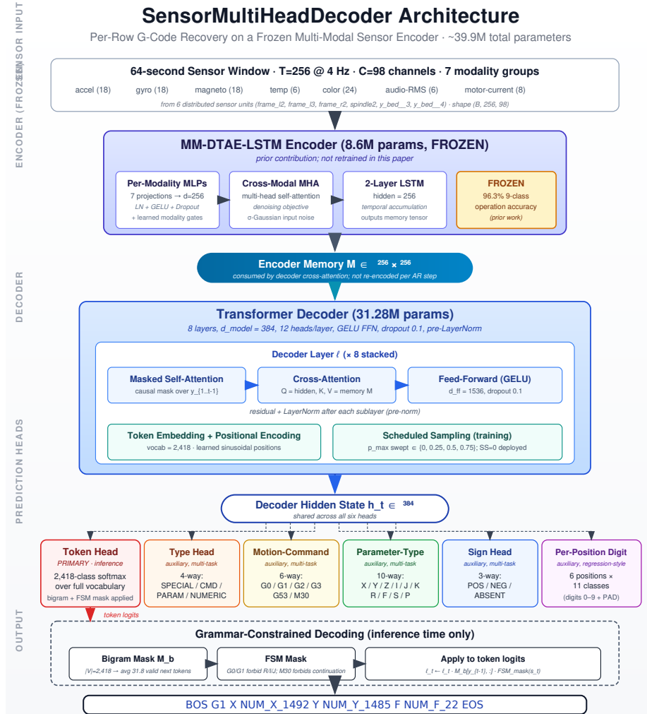
Figure 1. System overview. A 64-second sensor window (256 samples × 98 channels across seven modality groups) is mapped by the frozen MM-DTAE-LSTM encoder (8.6 M parameters) to a 256 × 256 memory tensor. An 8-layer Transformer decoder ( d_{\text{model}}=384 , 12 heads) consumes this memory via cross-attention and generates tokens autoregressively. Six prediction heads share the decoder’s hidden state and provide structured output (token, type, motion-command, parameter-type, sign, per-position digit). A static grammar mask zeros structurally invalid token transitions in the legacy-token softmax at inference time.
