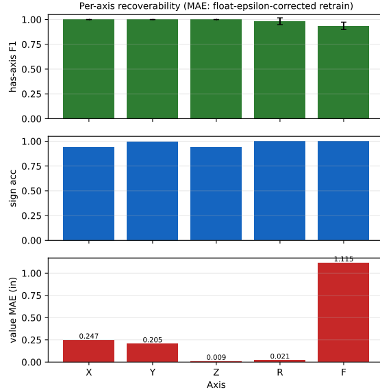
Figure S39: Per-axis G-code recoverability (5-fold mean): has-axis F1 (top), motion-sign accuracy (middle), and numeric-value MAE (bottom, inches). The categorical-vs-numeric split is visible: has-axis and sign reach high accuracy on the well-supported axes (X, Y, Z, R), while value MAE is the limiting factor for full coordinate reconstruction. The asymmetry in per-axis sign accuracies (Y \approx 1.00 vs Z \approx 0.94) reflects the near-deterministic sign prior on Y versus the genuinely balanced sign distribution on Z; the companion limit paper [Eacuella et al. (2026c) Eacuella, Prasad, and Sodhi] accounts for this through the per-axis sign-entropy decomposition.
