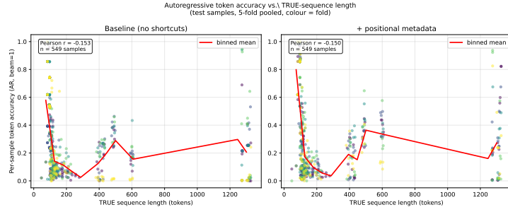
Figure S12: Per-sample AR token accuracy vs. TRUE-sequence length, pooled across 5 test folds. Pearson r \approx -0.15 in both configurations — a weak negative correlation: longer targets accumulate more exposure-bias error toward the corpus-modal sequence. Corroborating, not load-bearing.
