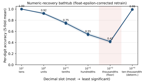
Figure S41: The numeric-recovery “bathtub”: pooled per-digit-position accuracy (5-fold mean \pm std, teacher-forced; float-epsilon-corrected retrain). Slot 0 is recovered at 1.00, accuracy descends monotonically to the precision floor at slot 4 ( 10^{-3} , thousandths; 0.42 — the finest digit the CAM postprocessor emits), and slot 5 ( 10^{-4} ) returns to 0.99 because the V8 tokenizer quantizes X/Y/Z onto a 0.001 grid, discarding the (near-uniform, \sim 3.31 -bit) source ten-thousandths digit; the tokenized target is therefore a structural zero reproduced trivially as a representation artifact, not an information-bearing recovery (companion paper [Eacuello et al. (2026c) Eacuello, Prasad, and Sodhi]). Source: audit/patched_numeric_analysis.json.
