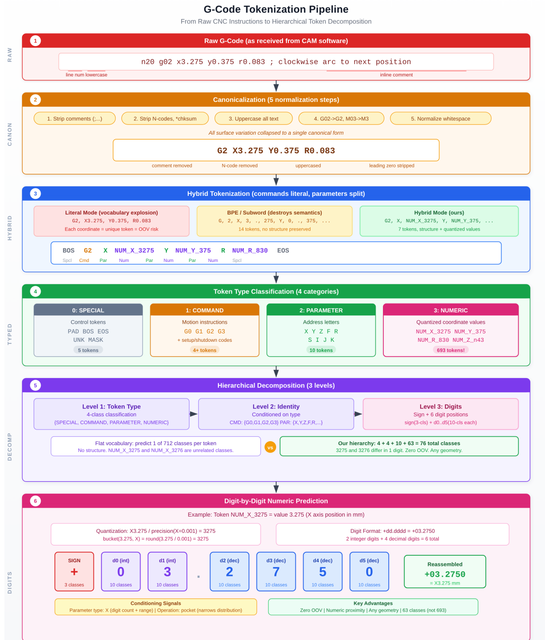
Figure A1. End-to-end tokenization pipeline. Raw G-code is canonicalized (5 steps), split into typed hybrid tokens, classified into 4 categories, decomposed hierarchically (3 levels), and predicted digit-by-digit (sign + 6 digits).
