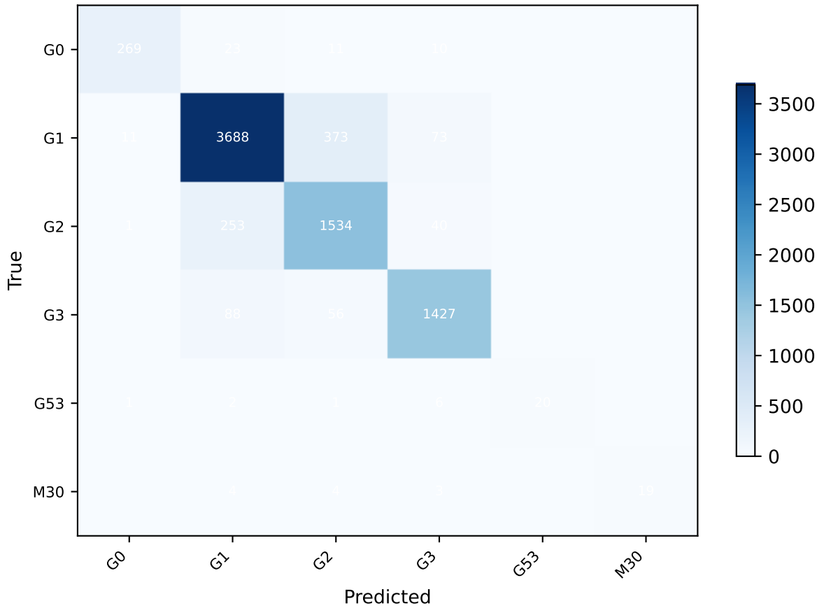
Command head — confusion matrix (5-fold aggregate counts)
