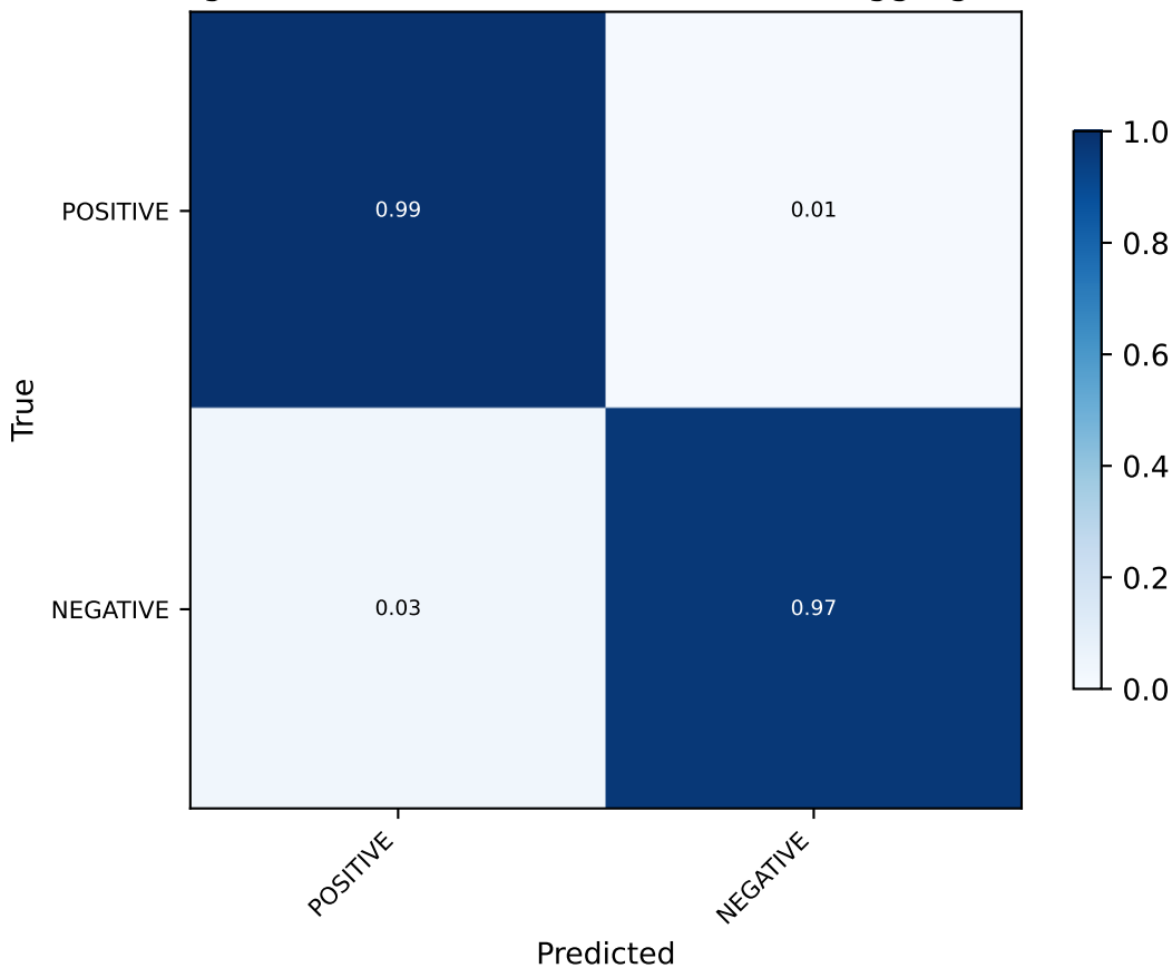
Sign head — confusion matrix (5-fold aggregate)
