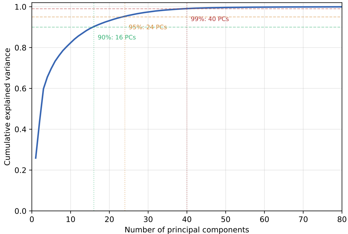
Effective dimensionality of the encoder memory (ambient D = 256 ; 24 PCs capture 95% of variance)
