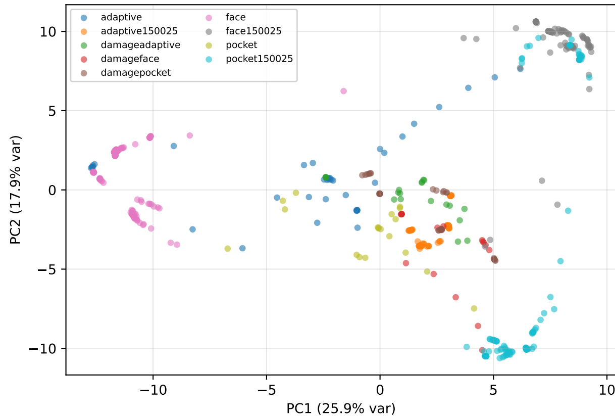
Linear PCA of mean-pooled encoder memory (colour = operation class)
