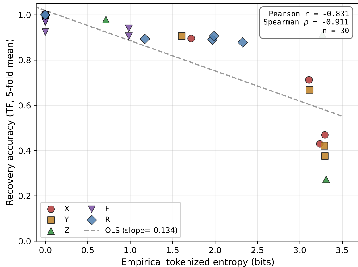
Per-(axis, slot) recovery vs. tokenized entropy ( n = 30 , patched)
