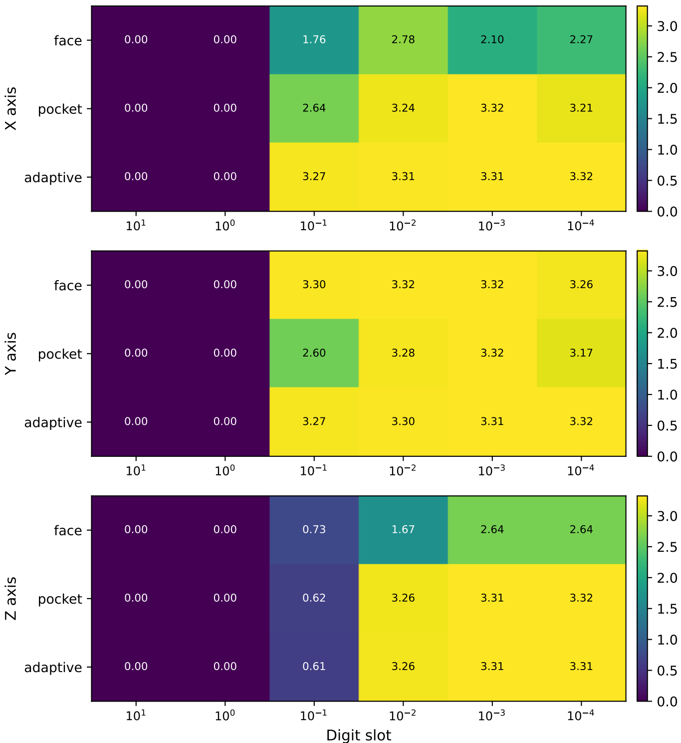
Per-axis per-slot per-op-family SOURCE entropy (bits)
