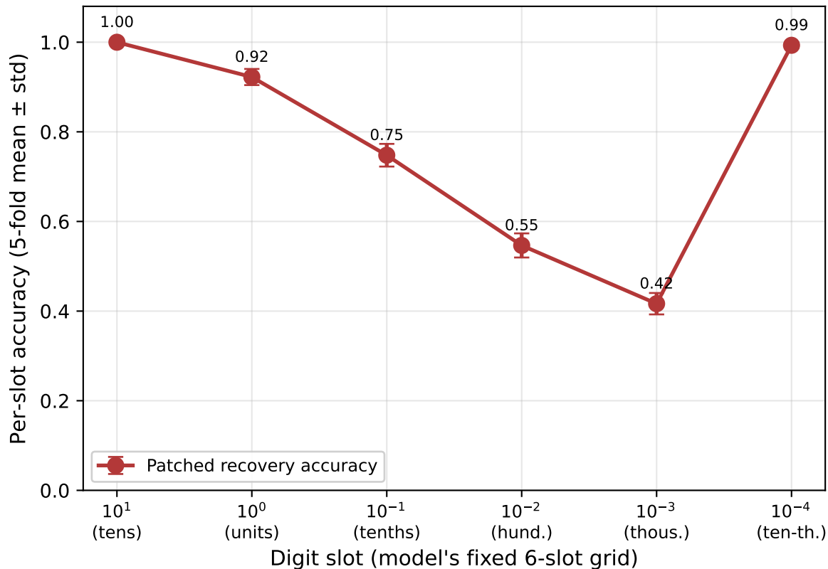
Pooled per-digit-slot recovery (patched encoder): the true precision floor is the thousandths ( 10^{-3} )
