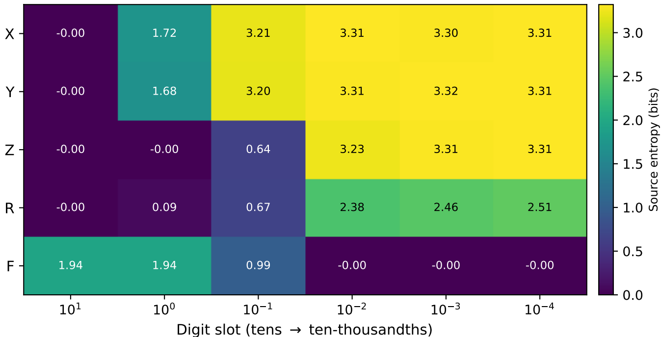
Per-(axis, slot) SOURCE entropy (bits); ceiling \log_2 10 \approx 3.32
