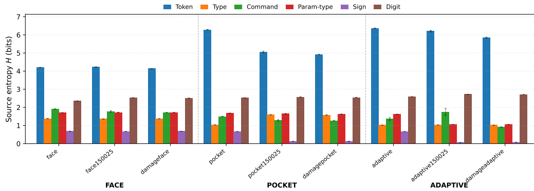
Figure 3. Per-toolpath empirical source entropy decomposed by prediction head across the nine operation classes, grouped by toolpath family (face / pocket / adaptive). The token head carries the largest absolute entropy; the digit head shows the cleanest facing-vs-adaptive separation: facing operations carry \sim 2.4 bits of digit-head entropy (overruns repeat workpiece-edge coordinates) while adaptive operations carry \sim 2.6 bits (near-uniform fractional digits). Sign and parameter-type heads are nearly toolpath-invariant. Regenerated from audit/per_head_per_opclass_entropy_5fold.json .
