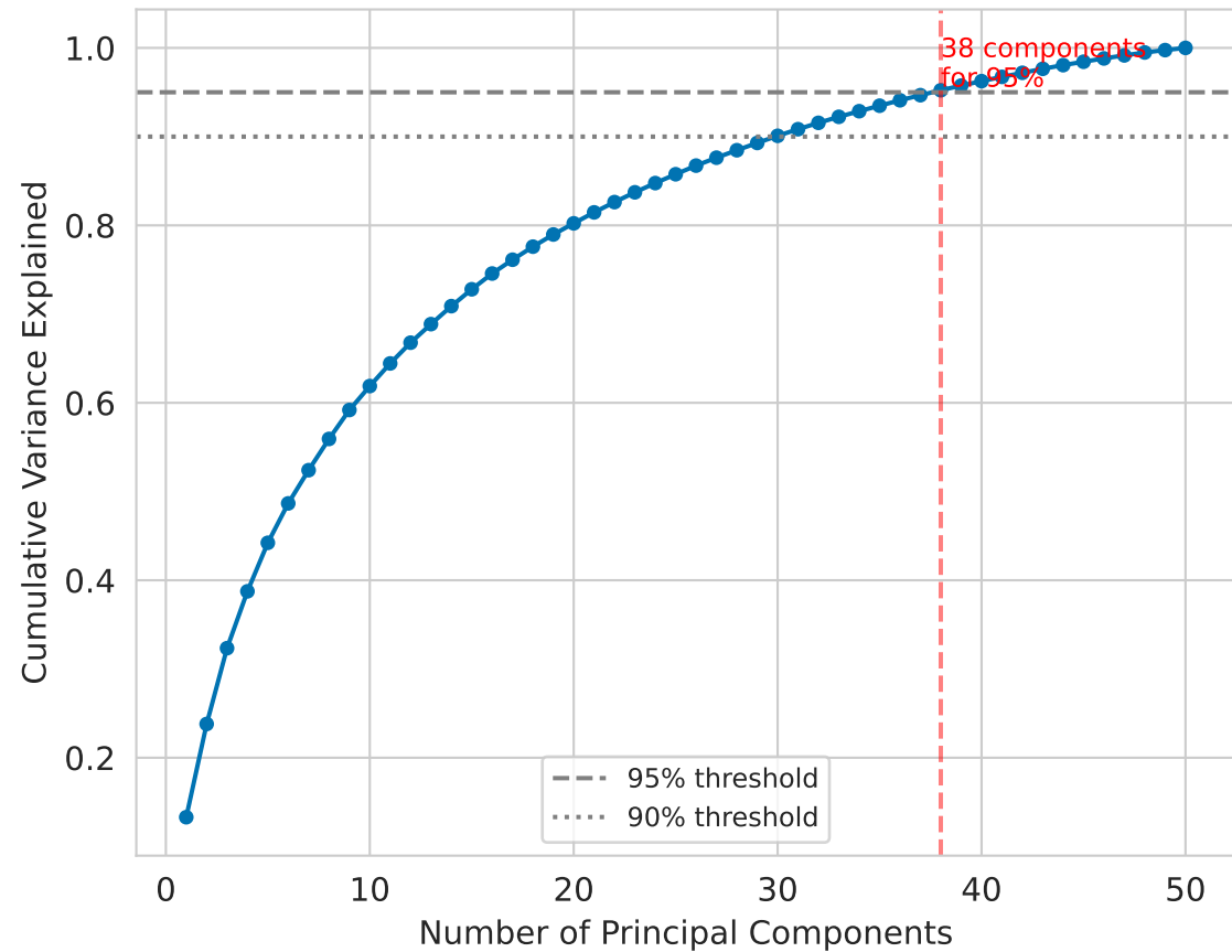
Scree Plot: Effective Dimensionality
