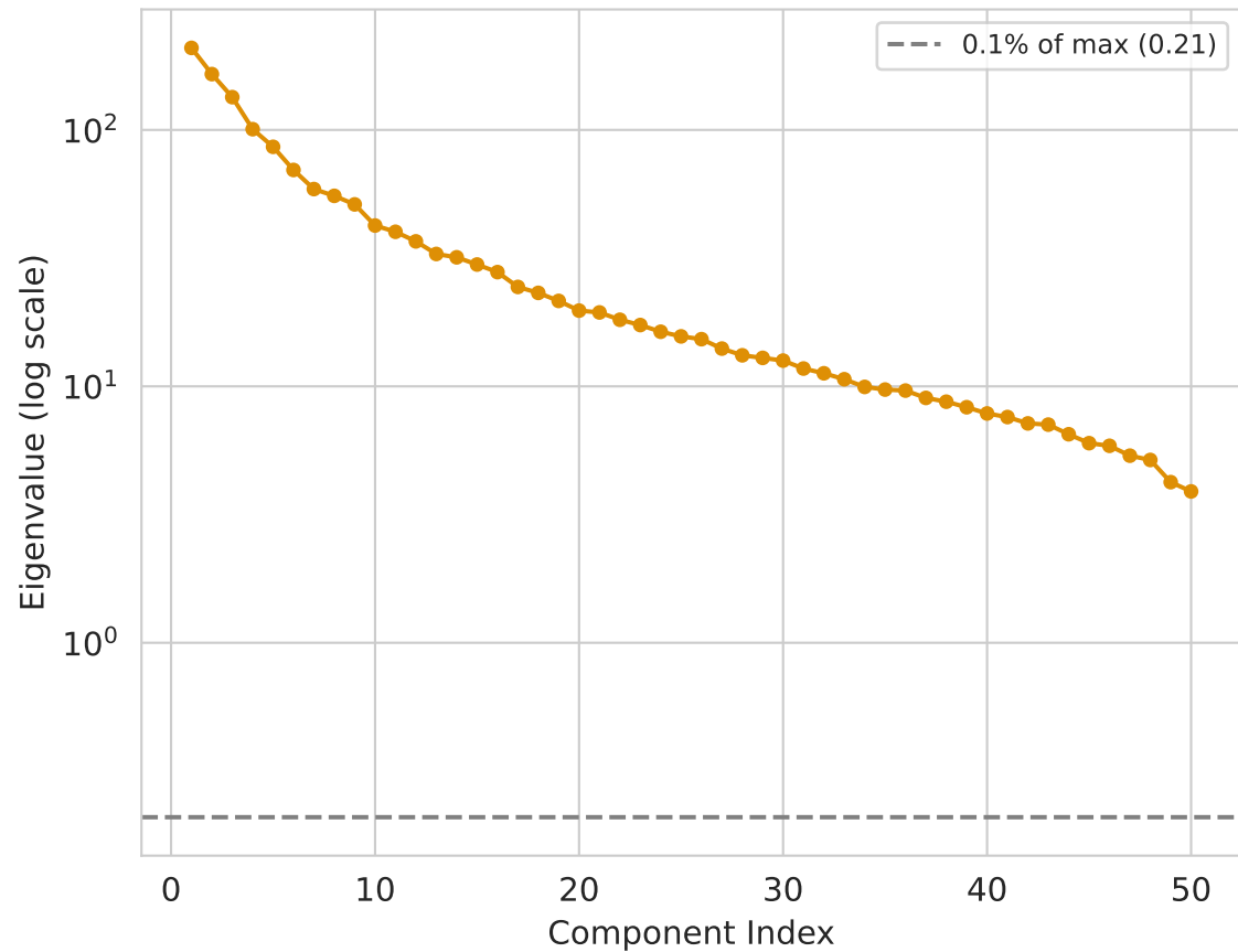
Eigenvalue Spectrum (effective rank = 50)
