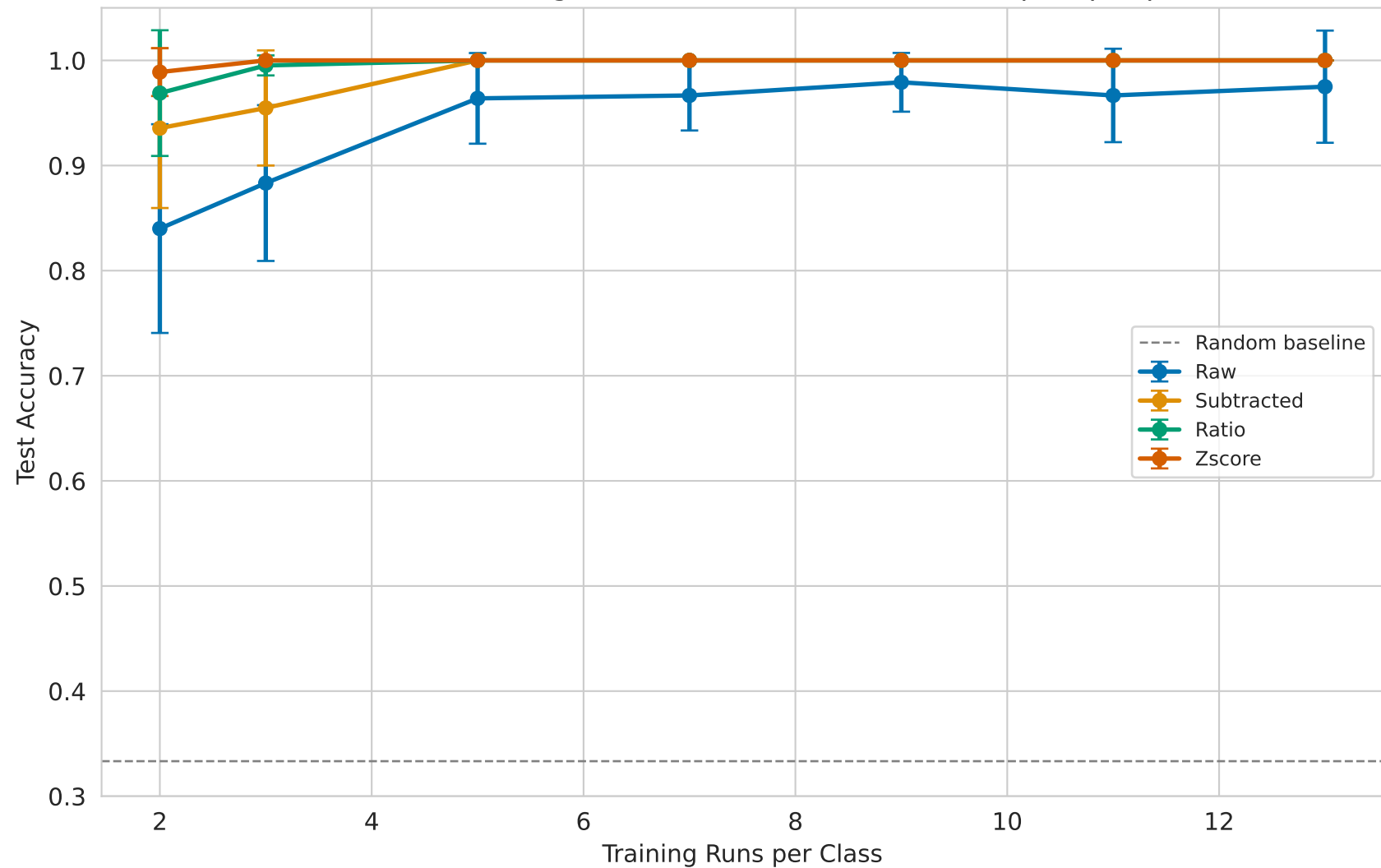
Fine-Grained Learning Curve (RF, 20 random subsamples per point)
