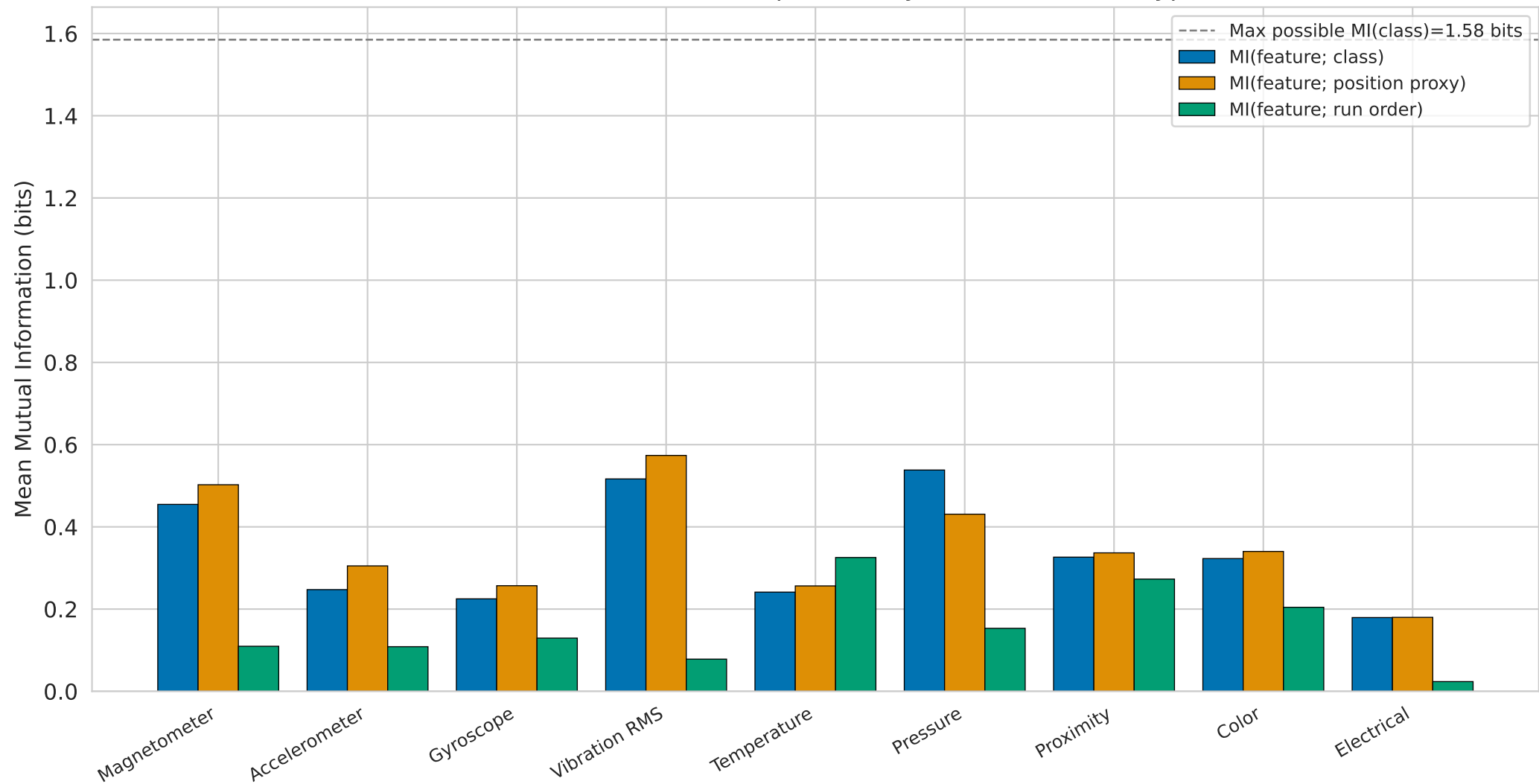
Mutual Information Decomposition by Sensor Channel Type
