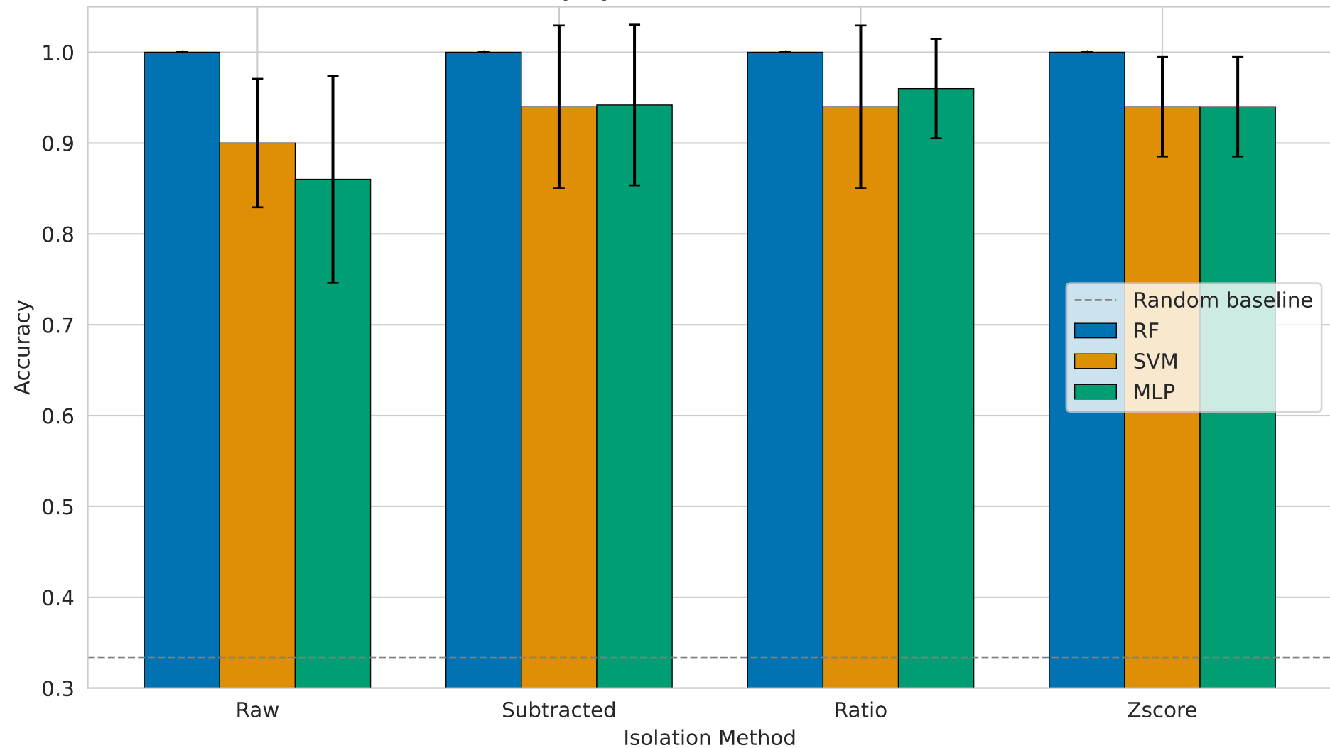
Classification Accuracy by Isolation Method and Classifier (No PCA)
