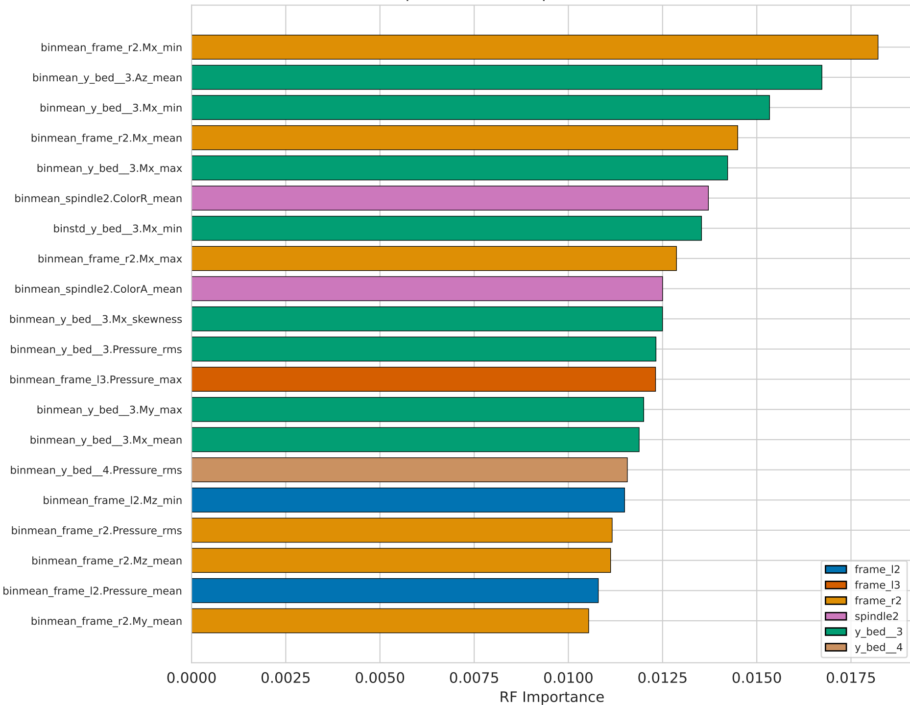
Top 20 Feature Importances (Raw, RF)
