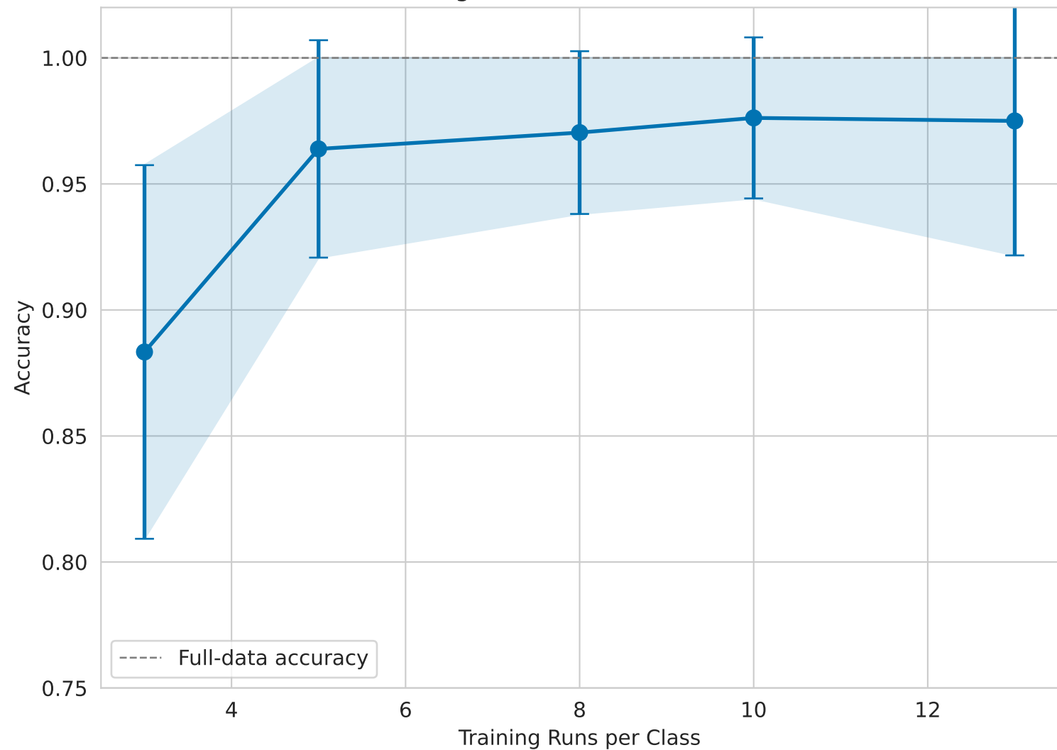
Learning Curve (RF, Raw Features)
