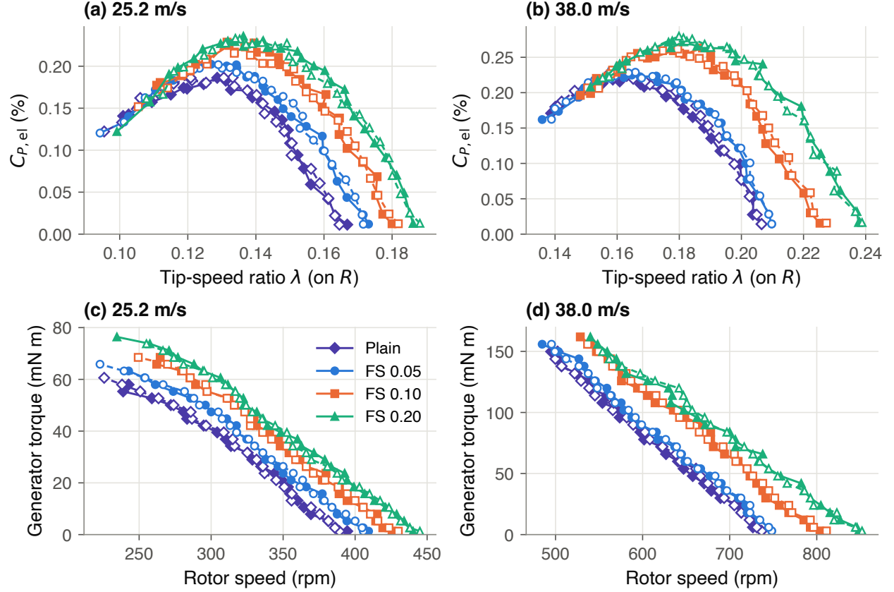
Figure 8. Electrical power coefficient against tip-speed ratio (a, b) and generator torque k_T I ( k_T = 0.30 \text{ N m/A} ) against rotor speed (c, d), from the speed at every load step; all eight runs (solid: run 1; dashed, hollow: run 2).
