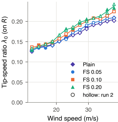
(a) Light-load tip-speed ratio
