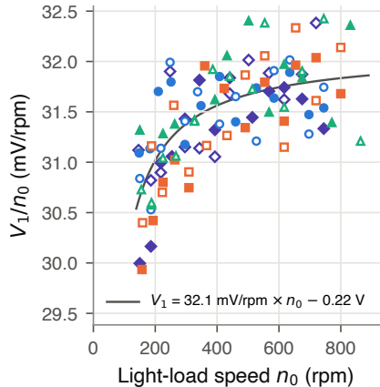
(c) Voltage per rpm
