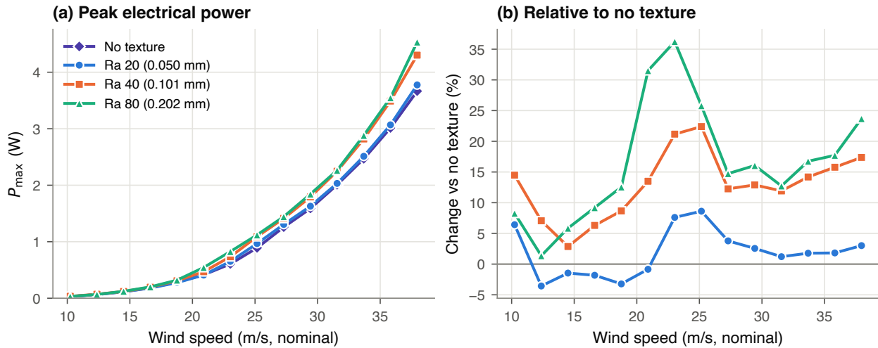
Figure 4. (a) Peak power against nominal wind speed, geometric mean of each rotor’s two runs. (b) The same relative to the un-textured rotor.
