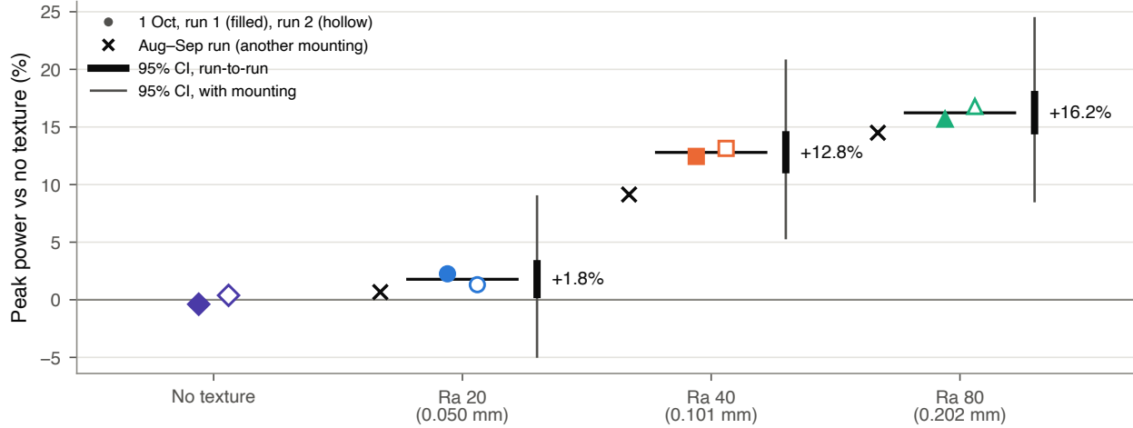
Figure 3. Peak power of every run relative to the un-textured rotor on 1 October (mean over 14 set points). Filled and hollow: the two 1 October runs on one mounting. Crosses: the August–September run, another mounting and day. Bars: rotor mean with 95% intervals, run-to-run (thick) and with mounting variation (thin).
