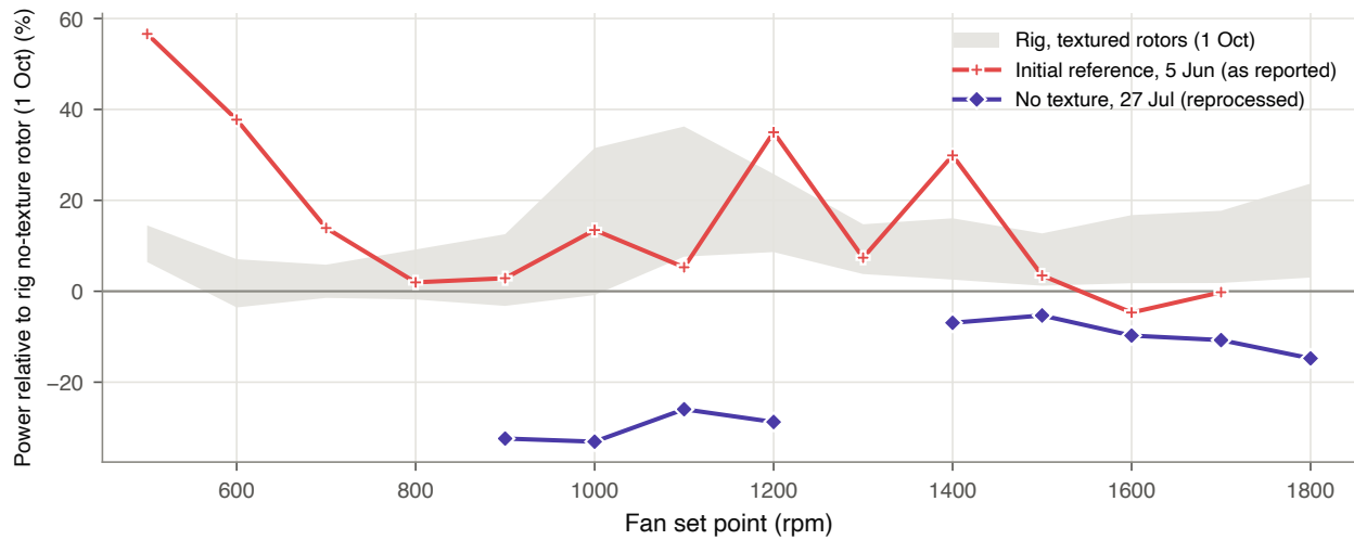
Figure 6. Jeong-lab tests relative to the rig’s un-textured rotor (1 October) at the same fan set point. Grey band: the rig’s textured rotors. 27 July: reprocessed (Appendix C); 500–800 rpm omitted (load off, or far below the power peak) and 1300 rpm (window spans a speed step). 5 June: as tabulated by the lab.
