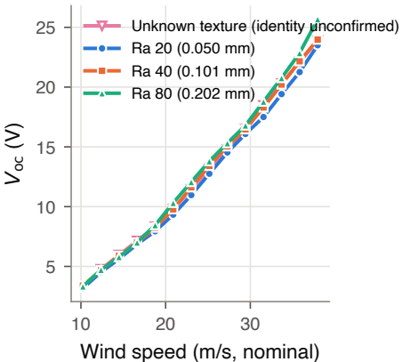
(a) Open-circuit voltage
