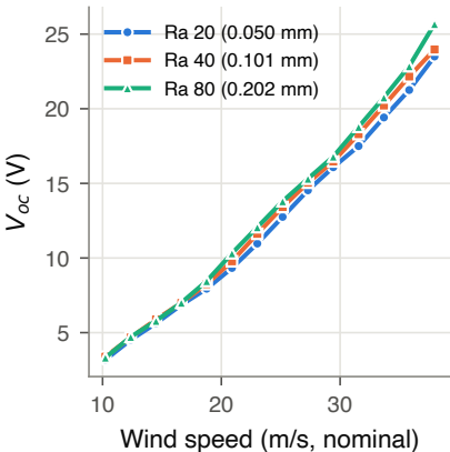
(a) Open-circuit voltage
