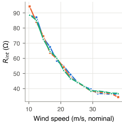
(b) Source resistance
